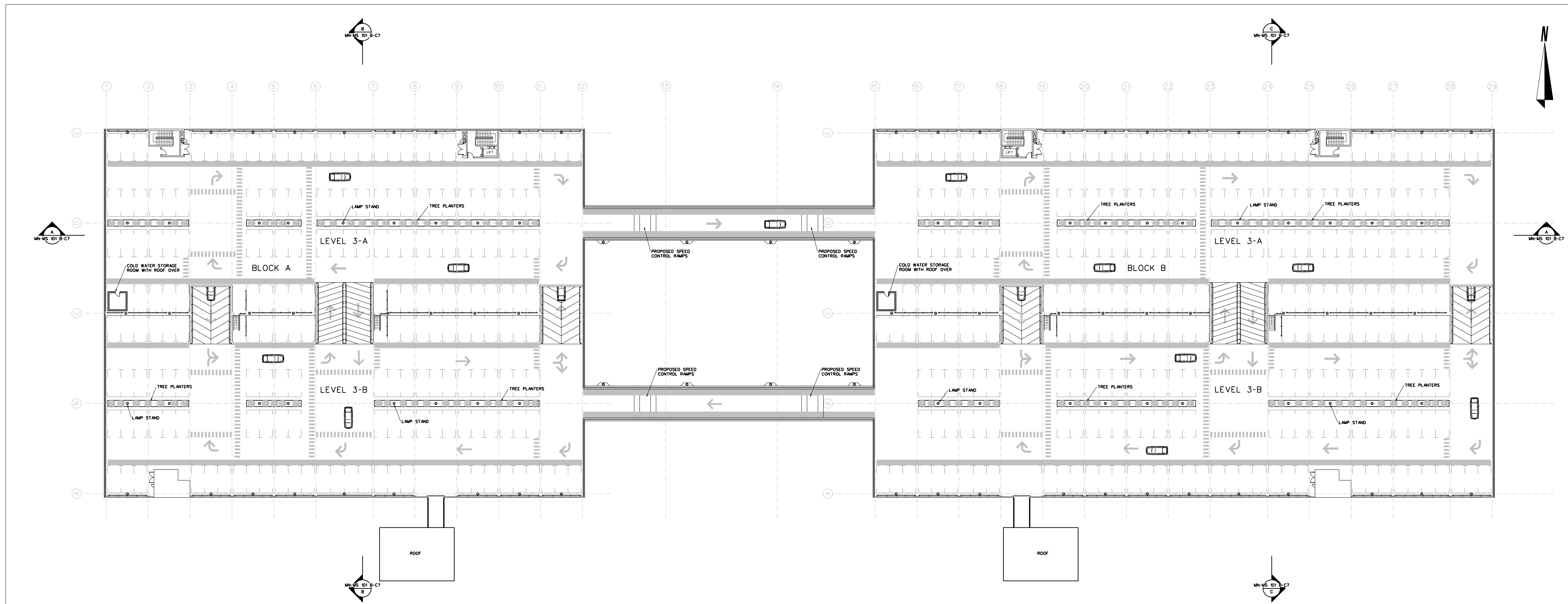
MULTI STOREY CAR PARK - LEVEL 3 PLAN SCALE 1:250
