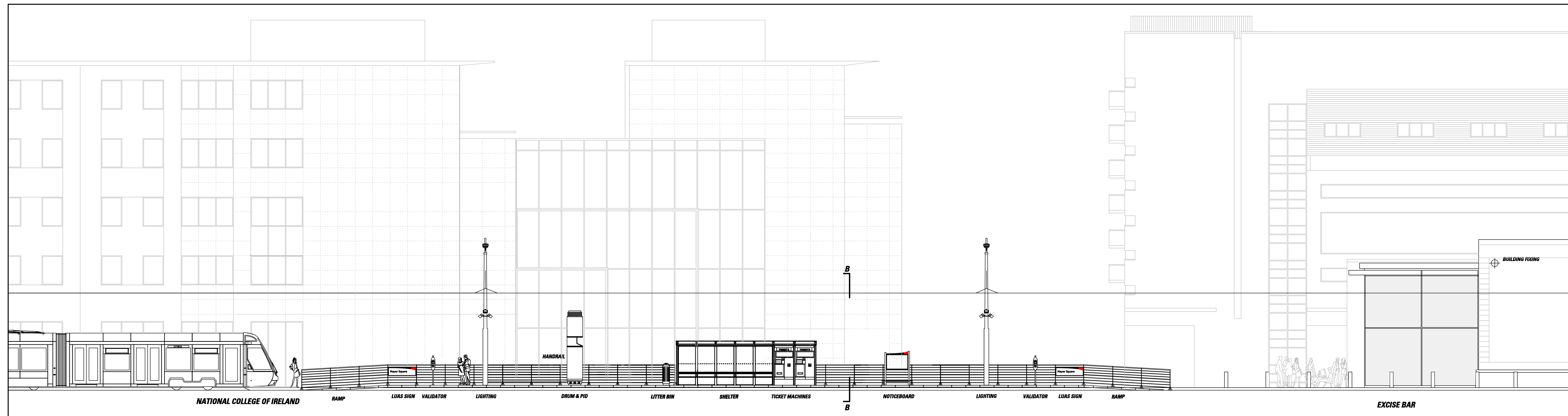
SECTIONAL ELEVATION AA SCALE 1:100
