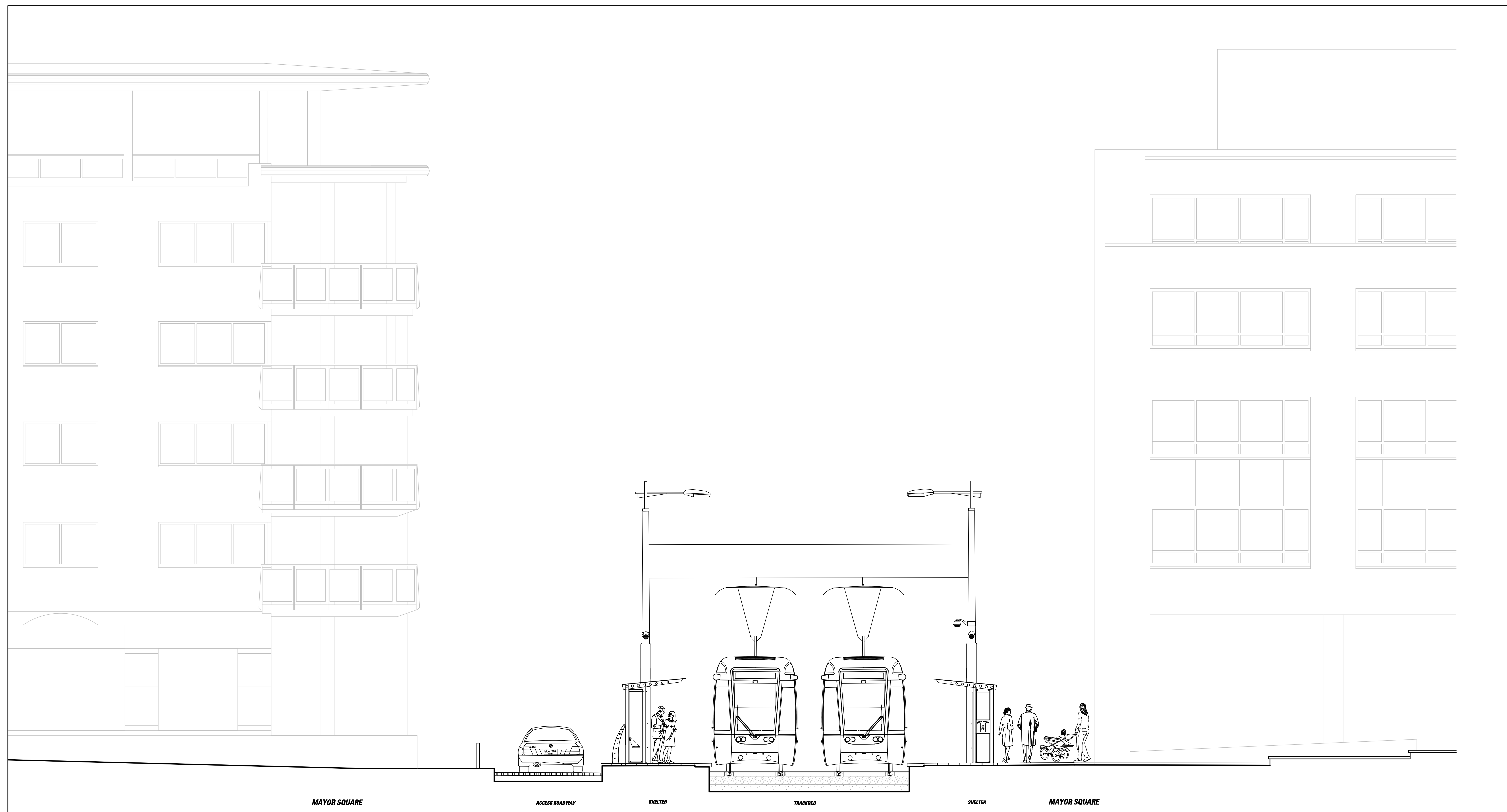
SECTION BB SCALE 1:50
